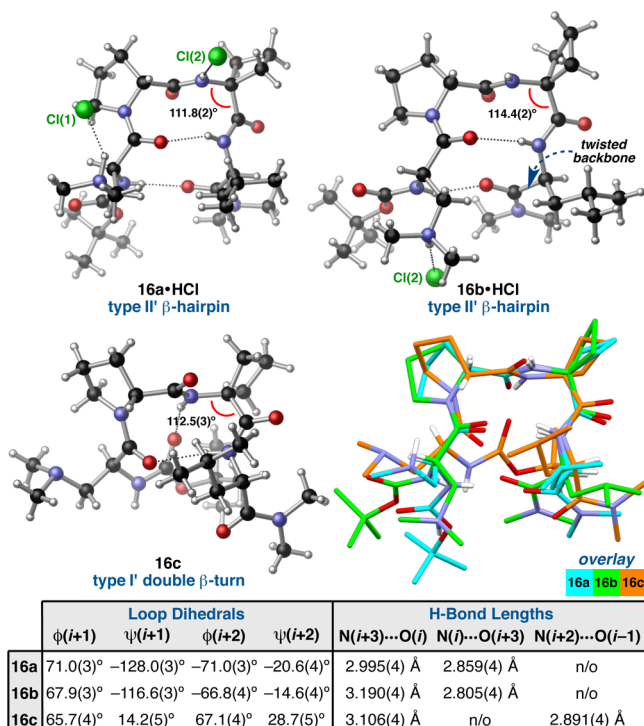
Figure 5. Three distinct conformations of peptide 16 with relevant crystallographic measurements. A structural overlay highlights the differences among the conformers (loop RMSD ( 16a/16b ) = 0.11 Å, loop RMSD ( 16a/16c ) = 0.74 Å).
